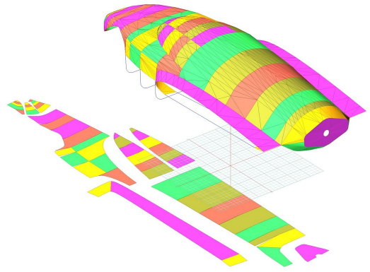
Cozy MkIV Canopy/Nose/Engine Cover, 3D model
