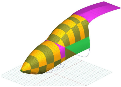
Laister LP-49 Canopy/Nose Cover, 3D model
