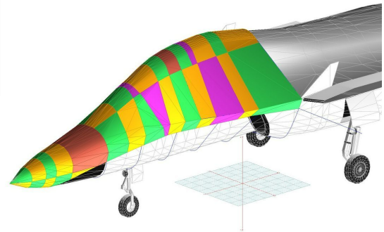
Aermacchi M-346 Canopy/Nose Cover, 3D model
