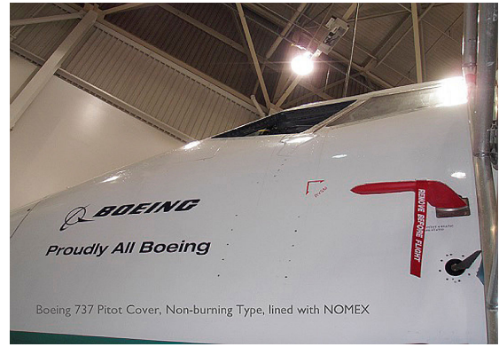
PITOT COVER
