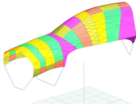
SAW Revo Canopy Cover w/fwd extension, 3D model
