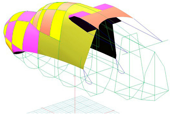
Schweizer 2-33A Canopy/Nose Cover, 3D model
