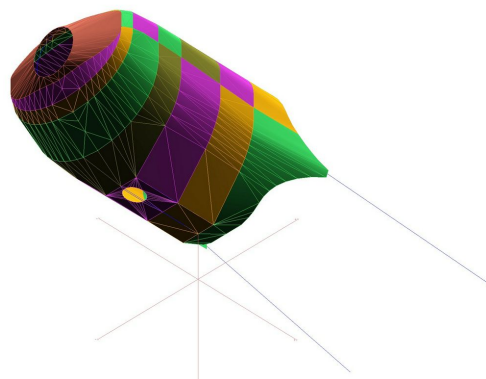
Socata TB30 Epsilon Insulated Engine Cover, 3D model
